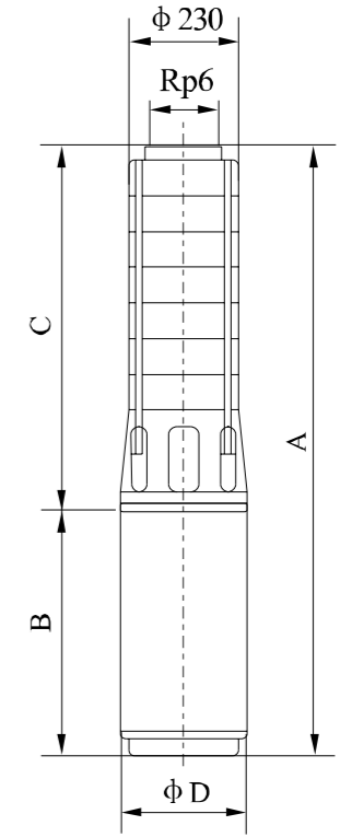
Installation sketch
